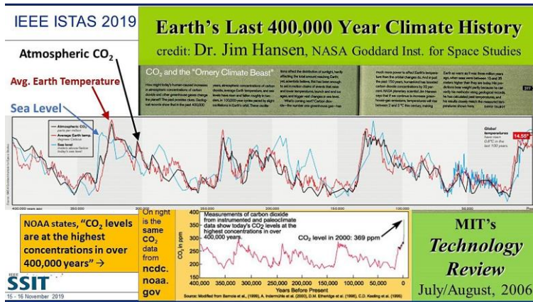
Fig. 4. Hansen graph correlating global CO 2 and temperature and sea level [10]
