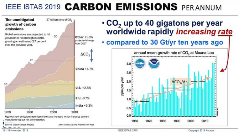
Fig. 2. Rate of change for CO 2 emissions per year [7]
