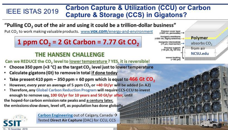
Fig. 13. Proposed CCS for excess atmospheric CO 2 to restore 20 th century 350 ppm levels [37]
