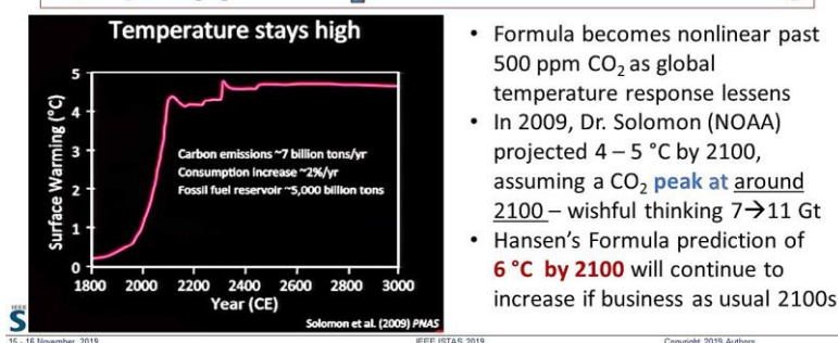
Fig. 7. Hansen formula with corroboration by Solomon et al. [14]
