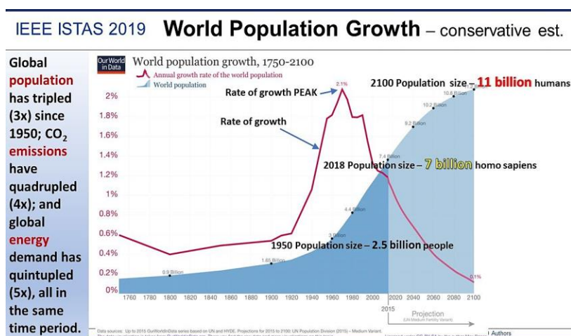
Fig. 1. World population growth [5]
