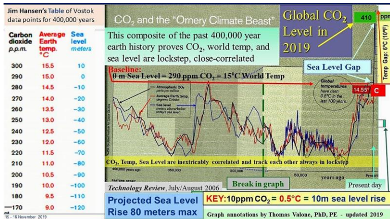
Fig. 5. Hansen's data table and interpretation of his graph by the author [11]
