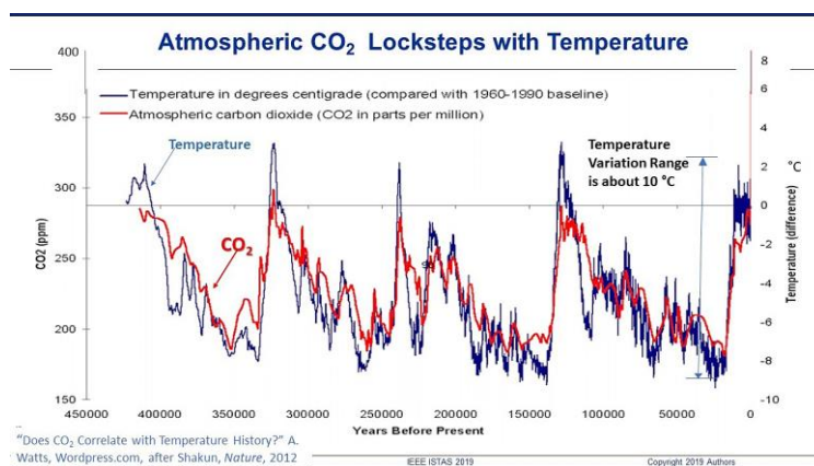
Fig. 3. Global average temperature tracks CO 2 levels [8]
