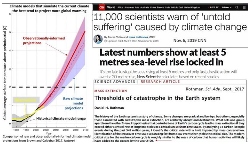
Fig. 8. Climate model simulation [17]
