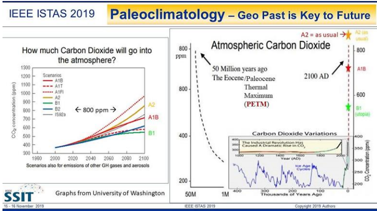
Fig. 9. Climate scenario model projections versus paleoclimatology [22]
