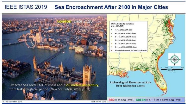
Fig. 10. Expected moderate increase in sea level from best estimates [25]
