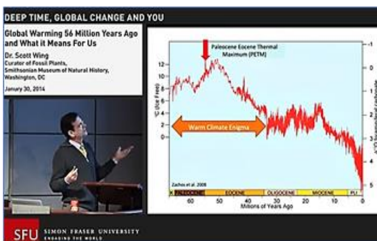
Fig. 11. Scott Wing explaining the PETM temperature maximum versus today's global warming climate [32]
