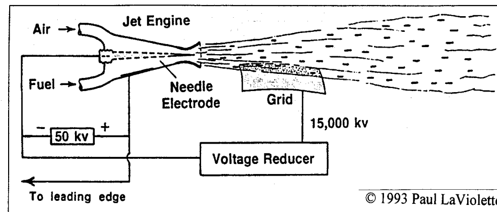
A high-voltage flame-jet generator.
